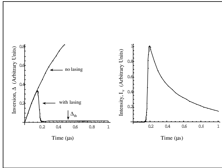
Figure 5. Solution of the laser rate equations for the inversion and laser intensity for a high gain, low optical loss system where chemical pumping of the upper laser level is initiated at t=0 .
