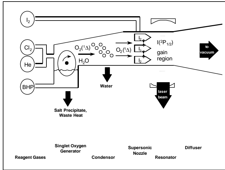
Figure 10. Schematic diagram of a typical supersonic Chemical Oxygen-Iodine Laser (COIL).
