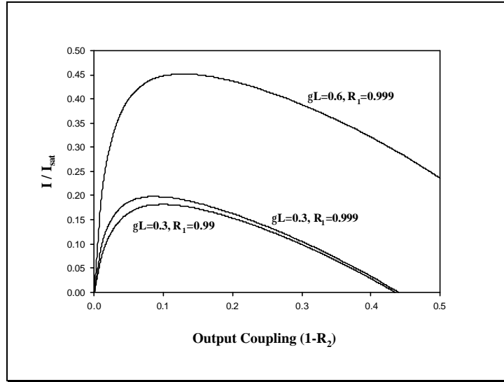
Figure 6. A Rigrod analysis of the laser intensity as a function of output mirror reflectivity, R_2 , for several values of gain and optical losses at the second mirror with maximum reflectivity, R_1 .
