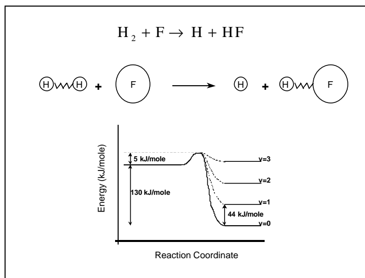
Figure 3. The reaction of atomic fluorine with molecular hydrogen produces vibrationally excited hydrogen fluoride. The reaction coordinate represents the breaking of the H_2 bond as the fluorine atom approaches and the subsequent formation of the HF bond as the product hydrogen atoms depart the collision center.
