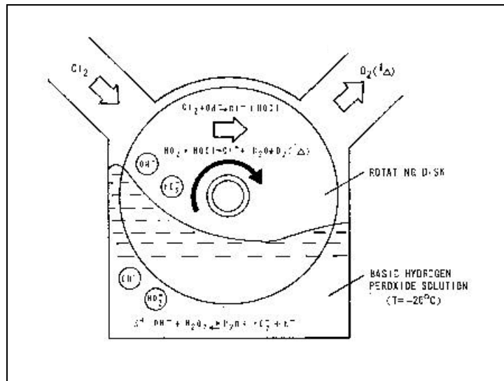
Figure 11. Rotating disk design for the chemical generation of singlet oxygen, O_2(a^1D) , via the two phase reaction of chlorine gas with liquid hydrogen peroxide.
