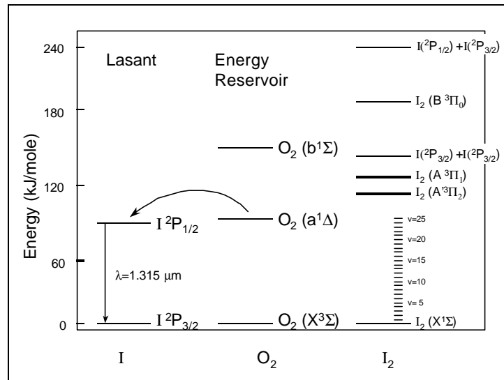
Figure 8. Energy level diagram for the Chemical Oxygen-Iodine Laser illustrating the resonant energy transfer from metastable reservoir O_2(a^1D) to the upper laser level of atomic iodine, I(^2P_{1/2}) . The energy levels for several key states involved in the dissociation of molecular iodine are also provided.
