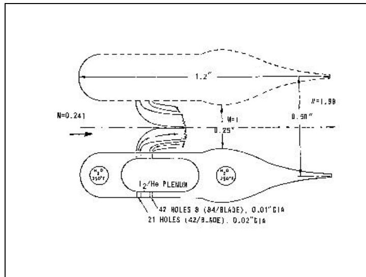
Figure 12. Typical supersonic mixing nozzle for a Chemical Oxygen-Iodine Laser where molecular iodine is injected transverse to the flow of singlet oxygen.
