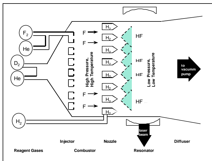
Figure 4. Schematic diagram of a typical supersonic mixing hydrogen fluoride chemical laser.
