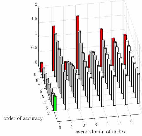
Figure 12: The Gregory weights near the left end of an interval, for increasing orders of accuracy (2, 3, 4, ..., 9). Trivial weights (with the value one) are shown as white bars that also continue to the right of what is shown. Where color is available, the front row displaying the nontrivial weight \frac{1}{2} of the trapezoidal rule is indicated with a green bar and the nontrivial weights for the bottom row of table 1 are illustrated in red.
