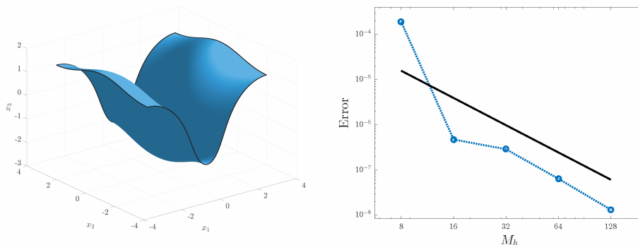
FIG. 3.2. Left: A relatively large amplitude wave, h=4.23 , used for the convergence study on the right. This wave has At=1, g=-0.1, \tau=2 . At larger amplitude and transverse variation this wave overturns, and is depicted in figure 3.4. Right: The Cauchy error of the computed wave speed, |c(M_b) - c(2M_b)| , is plotted as a function of points in the \beta coordinate M_b (marked with circles). The number of points in the \alpha direction is fixed at M_a=256 . The solid line is O(M_b^{-2}) .
