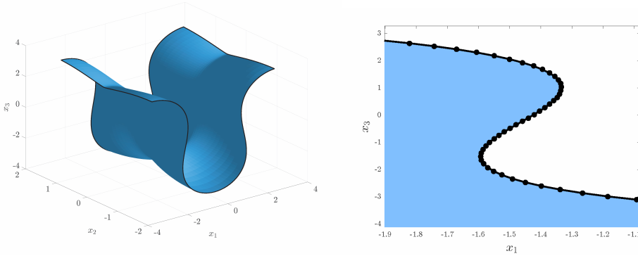
FIG. 3.4. An overturned fully three-dimensional traveling wave solution to (2.6), using the small-scale approximation to the Birkhoff-Rott integral. This wave was computed with At=1, \tau=2, g=-0.2 , with M_a=128 and M_b=32 . In the left panel is the three-dimensional surface, in the right panel is a close-up of a slice at y=-\pi/2 . In the close-up on the right, the grid-points are marked with solid circles.
