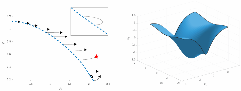
FIG. 3.1. The dimension breaking bifurcation of traveling waves solutions to equations (2.6) is depicted in the speed, c , and total displacement, h = \max(z) - \min(z) , plane. The waves bifurcate from a planar wave with Bond number \sigma = 1/8 , whose speed-amplitude curve is marked with the dashed curve in the left panel. The secondary, dimension-breaking bifurcations occur at different amplitudes depending on the transverse period (the secondary bifurcation's speed-amplitude curves are marked with arrows at their tips). Notice that there is closed loop, representing a “return to trivial” global bifurcation, a close-up of this loop is inset. An example genuinely three-dimensional profile, marked with the star in the left panel, is depicted in the right panel.
