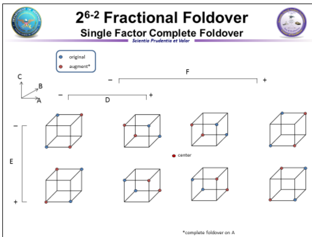
Figure 4: A Fractional Factorial Design + Fold Over example (Blue dots represent the original design and red dots represent the fold over design points)
