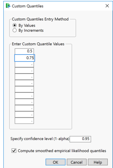
Figure 2: JMP Instructions Step
