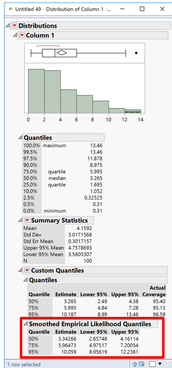
Figure 5: JMP results for sample of size n = 100
