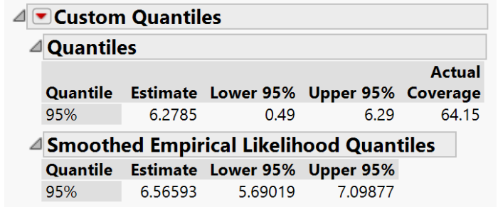
Figure 4: JMP results for 95 th percentile
