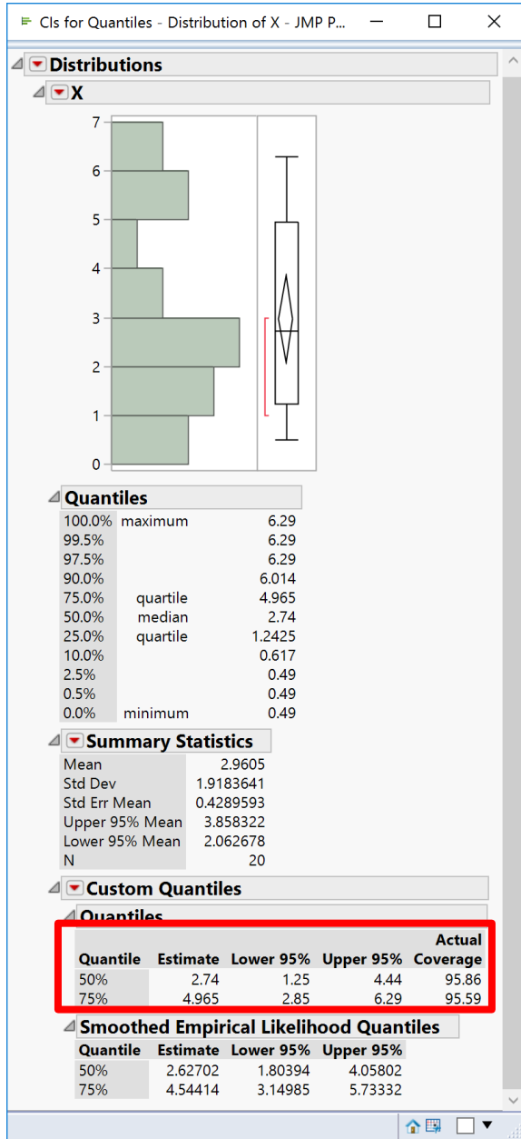
Figure 3: JMP Output
