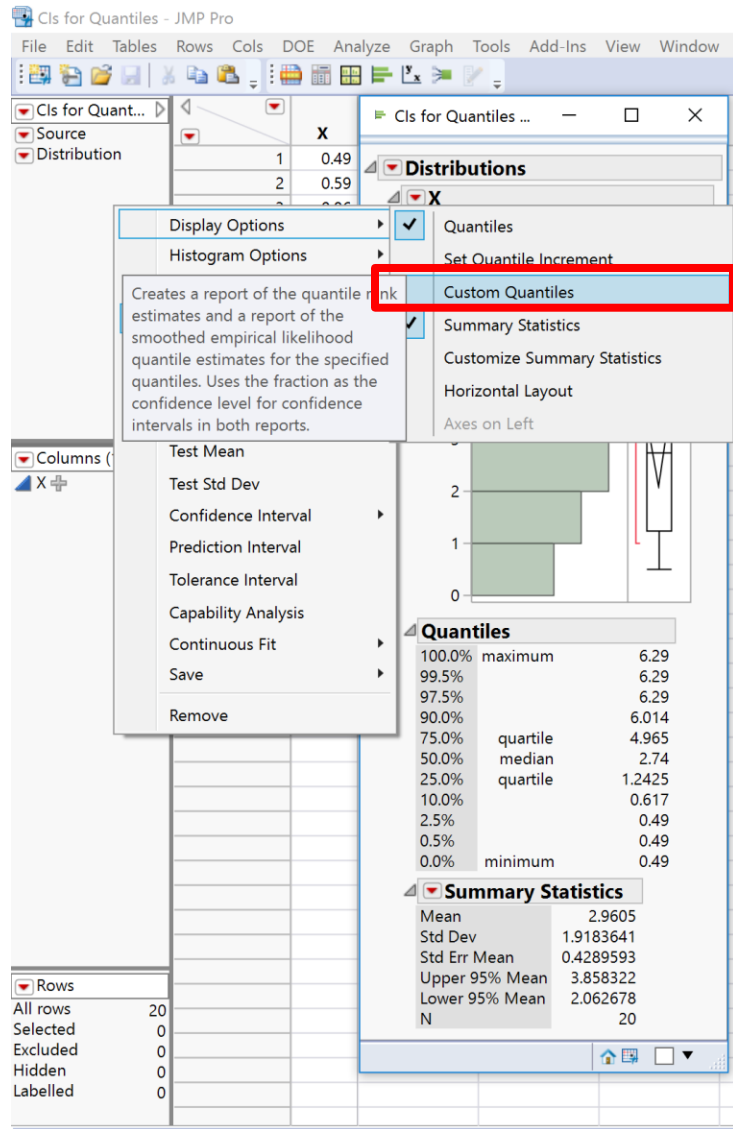
Figure 1: JMP Instructions Step 1
